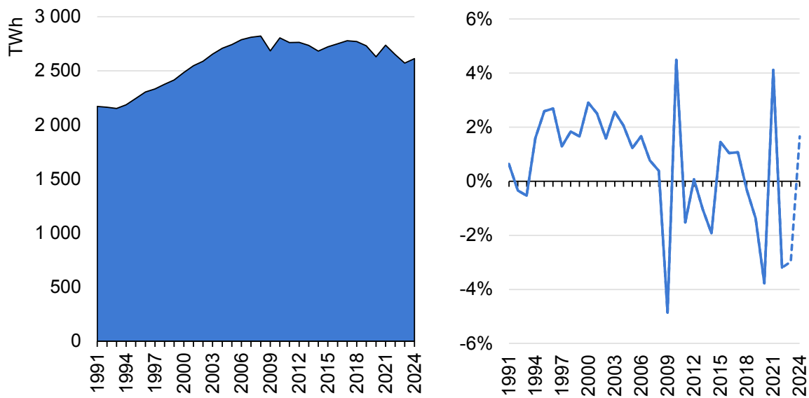
Evolution of electricity demand in the European Union (left) and its year-on-year percent change (right), 1991-2024
